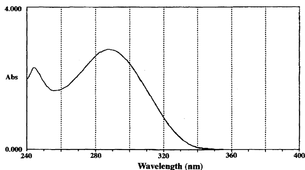
Fig. 6. UV/vis spectrum of 1 ( \text{CDCl}_3 as solvent).
