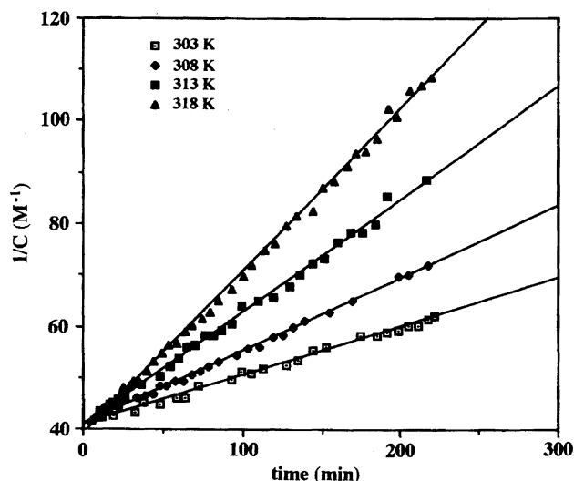
Fig. 8. Second order kinetics of the dimerization of 1 for a 0.024 M \text{CDCl}_3 solution at 303, 308, 313, and 318 K.
